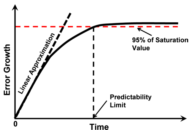
Fig. 1 Schematic illustration of the determination of the predictability limit from the mean error growth as a function of time, obtained using the NLLE method. The mean error growth on the y-axis uses a logarithmic scale to amplify the differences between linear and nonlinear error evolutions
